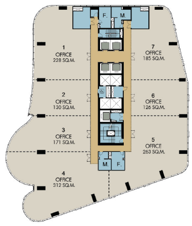
TYPICAL FLOOR PLAN Start From 130 – 1,500 sq.m.
